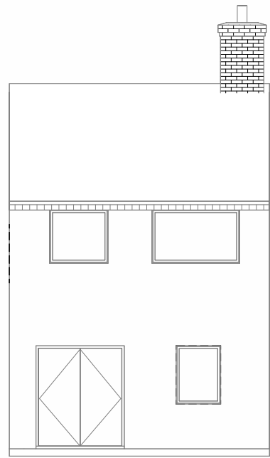
2 Existing Rear Elevation 1 : 50
