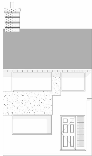
1 Existing Front Elevation 1 : 50
