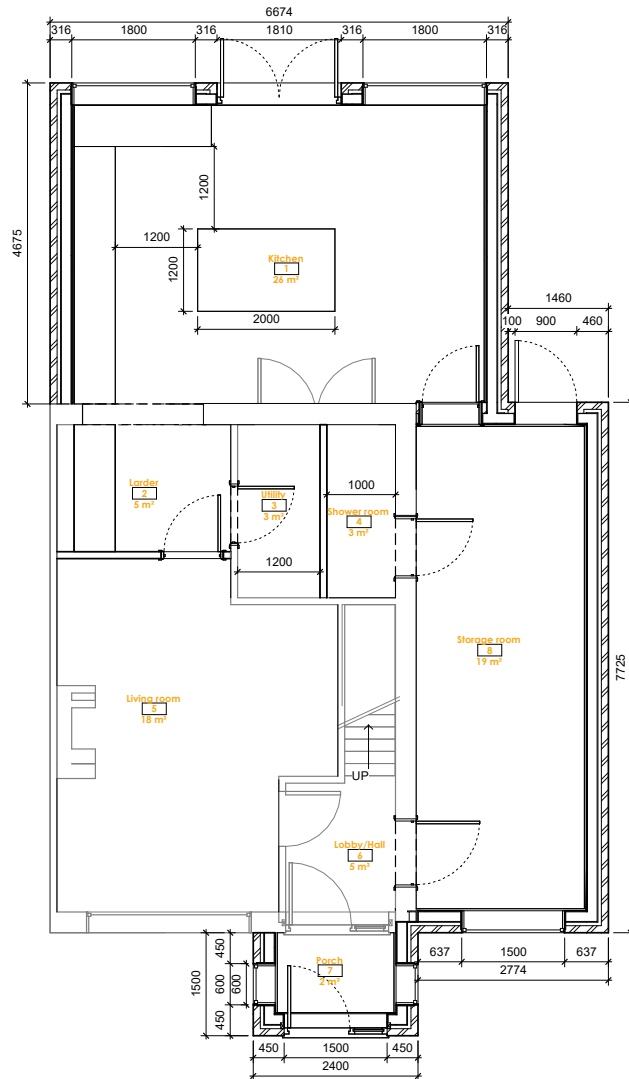
4 00 Proposed Ground Floor Plan 1 : 50
