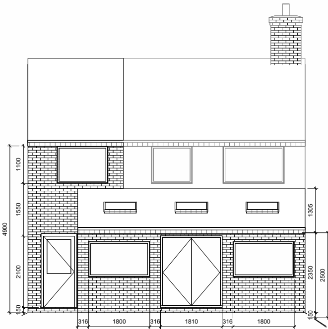
5 Proposed Rear Elevation 1 : 50
