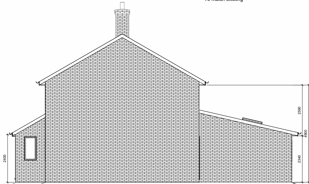
6 Proposed Side elevation 1 : 50
