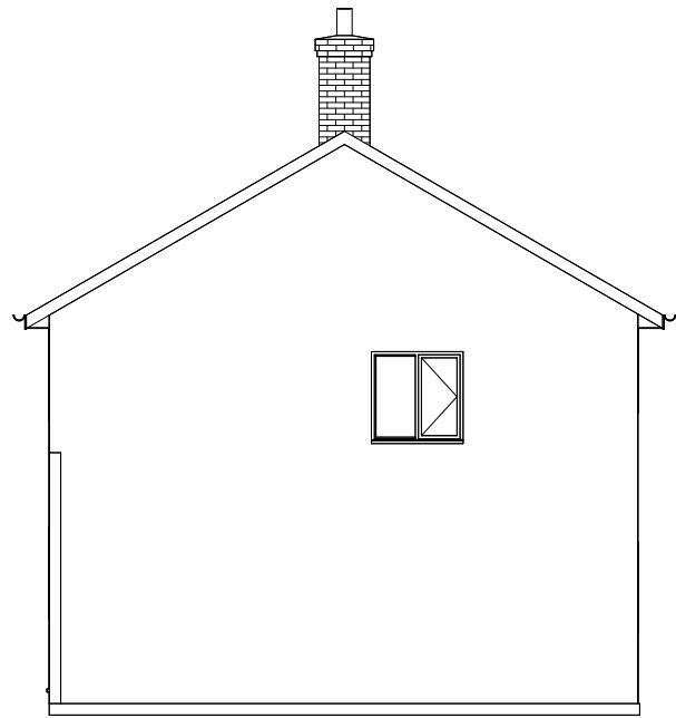
3 Existing Side elevation 1 : 50
