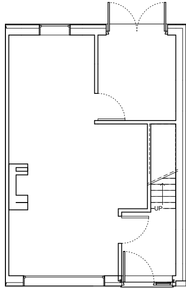
1 00 Existing Ground Floor Plan 1 : 50
